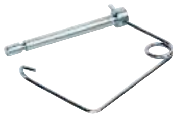
2-Pk. Handle Lock Hitch Pins Positive locking. Spring made of steel wire and swivels on head. All parts are zinc-plated and chromium lusterized to prevent rusting. Pin 1/4" dia., usable length is 1-3/4". 716201 $5.29 1/4" x 2-1/8" 716210 $5.29 5/16" x 2-1/4" 716229 $6.49 5/16" x 2-1/2" 716238 $6.49 3/8" x 1-1/2" 716247 $7.49 3/8" x 2-3/8" 716256 $7.79
